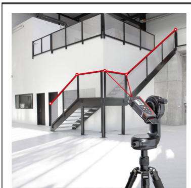
Point to point meting
